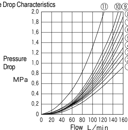
Pressure Drop Characteristics
