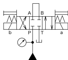
[Circuit Example]
