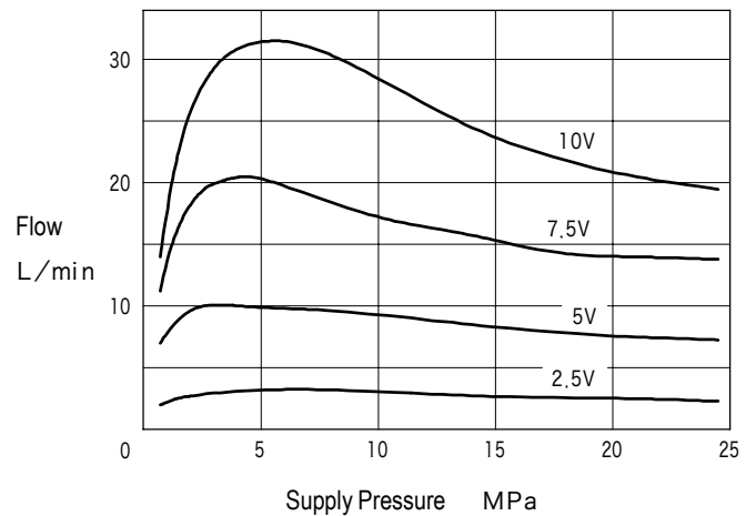
Supply Pressure - Flow Characteristics
