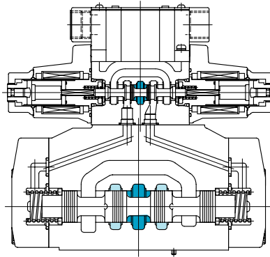
DG5V-7/H8-*A Spring Offset, A Type
