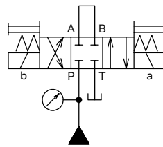
[Circuit Example]
