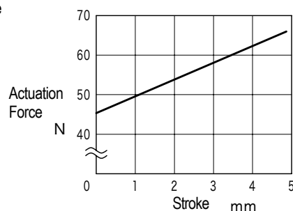
Actuation Force
