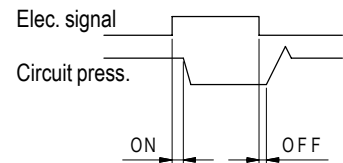
[Switching Time Definition]
