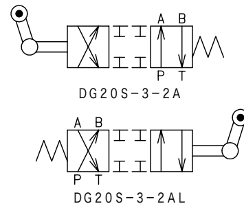
Functional Symbols
