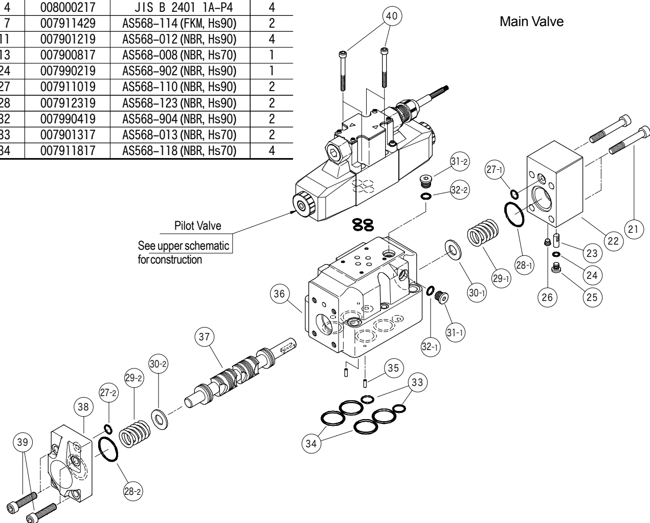
O-Rings COM-7
