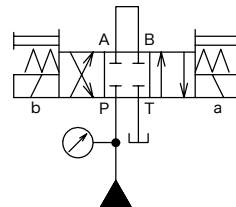
[Circuit Example]
