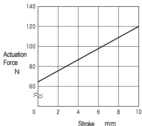
Actuation Force
