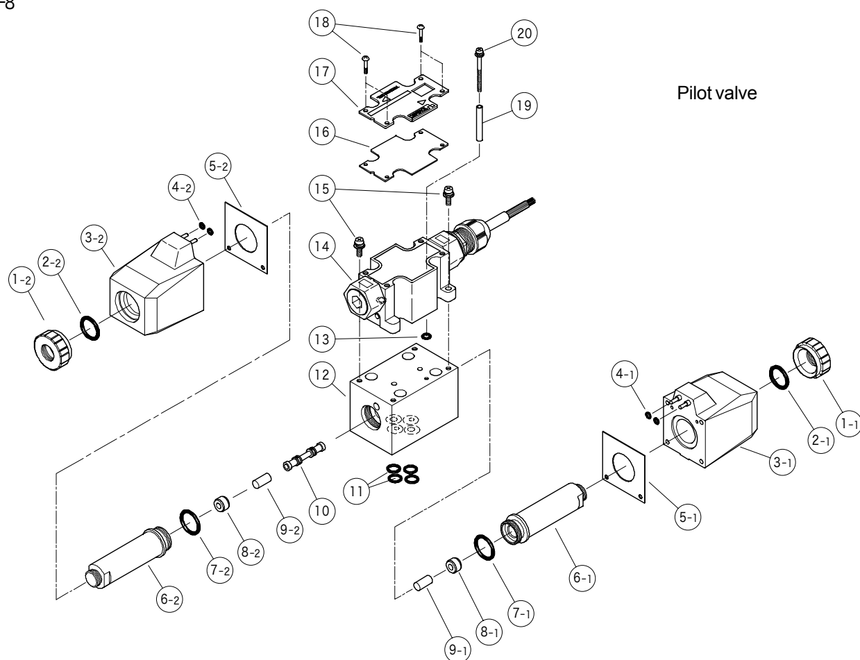
O-Rings COM-8
