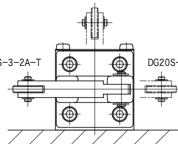
DG20S-3-2A-S
