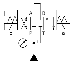
[Circuit Example]
