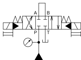
[Circuit Example]
