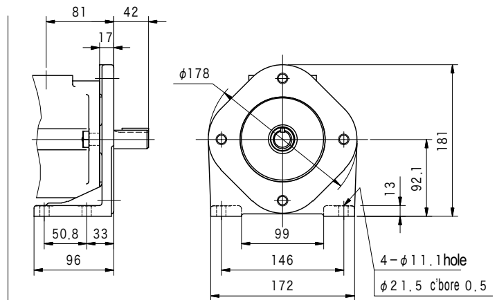
(Foot Mount)
