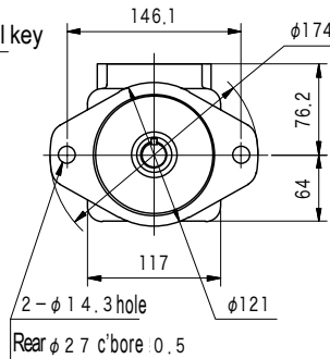
(Foot Mount)
