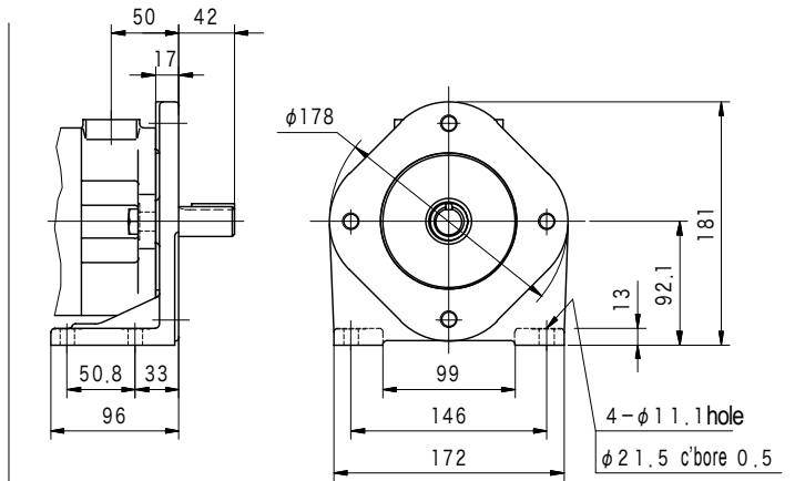
(Foot Mount)
