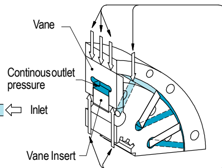
Fig.2 Shaft rotation causes alternate quadrant shifts in delivery load pressure and inlet suction pressures.
