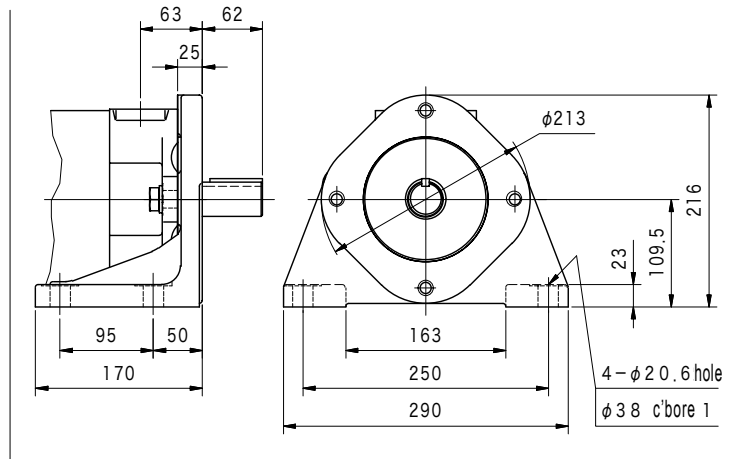
(Foot Mount)
